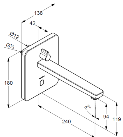
Dimensional drawing
